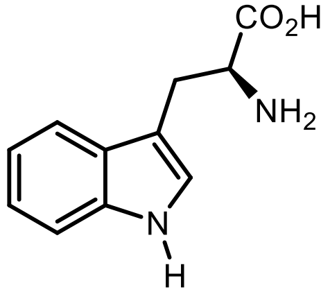
L -Tryptophan (Trp, W) proteinogene Aminosäure
